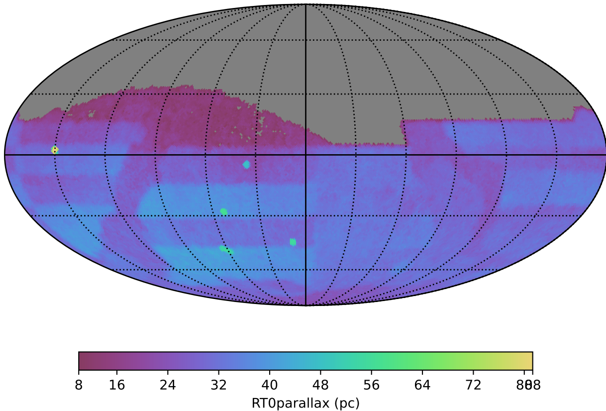
baseline_v5.3.0_10yrs night < 730: RT0parallax
