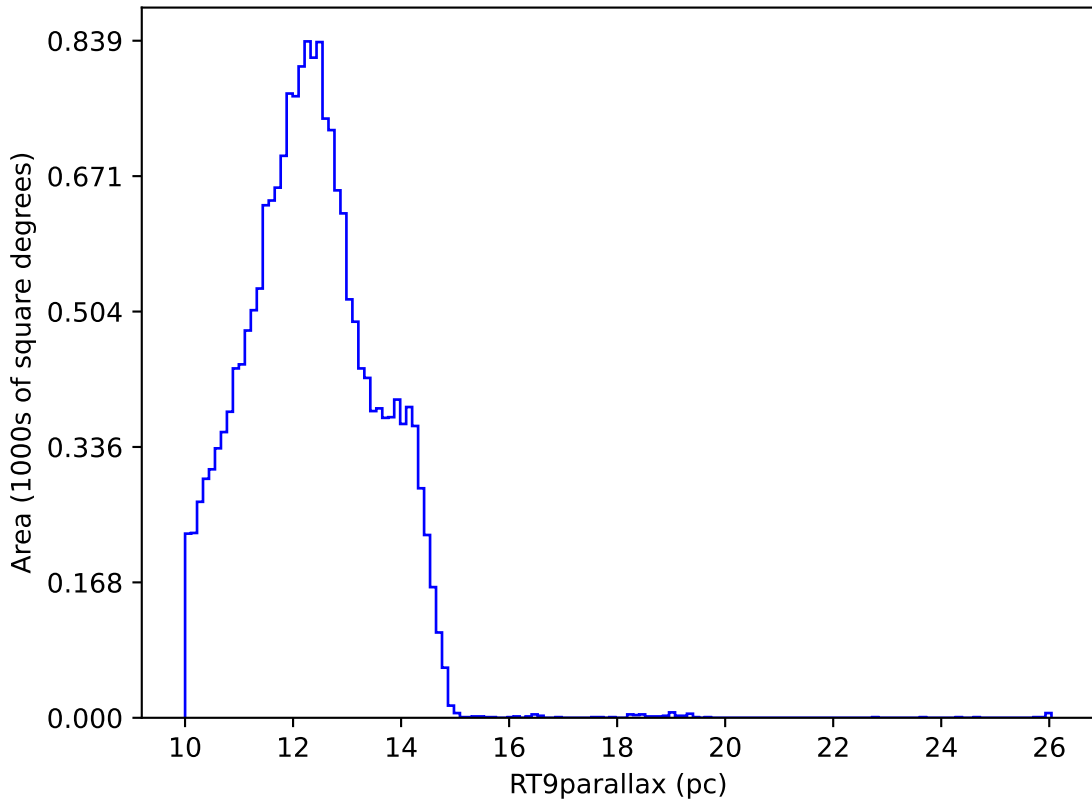
baseline_v5.3.0_10yrs night < 730: RT9parallax
