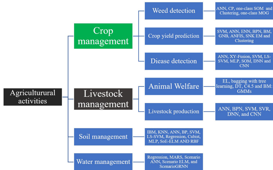
FIGURE 4 ML algorithms deployed for agricultural application
