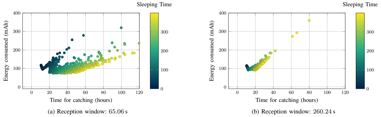
Fig. 2. Scatter plots showing the relationship between time for catching the beacon and energy consumed. Color intensity represents the sleeping time of nodes under two reception window configurations.
