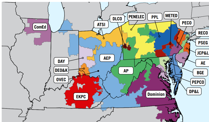
Figure 3.17: Map of PJM by Zones.
