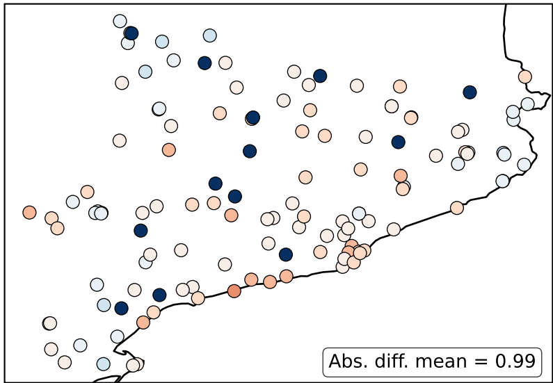
Pre-trained
