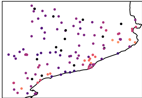
No pre-training
