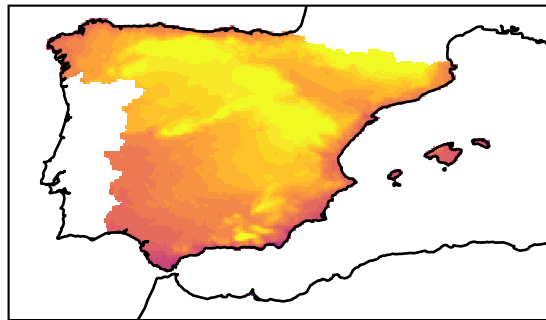
TNn
