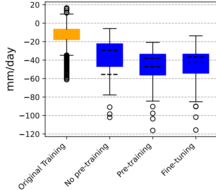
Bias Rx1day
