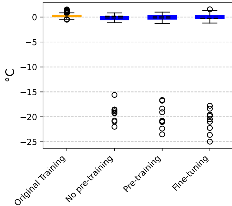
Bias Mean
