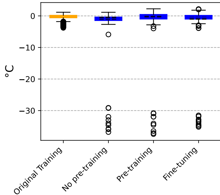
Bias TXx
