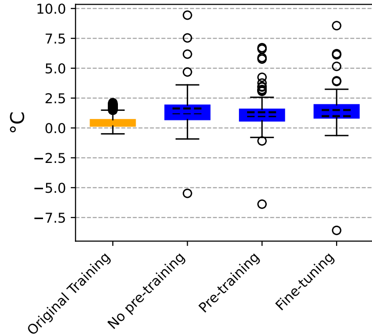
Bias TNn
