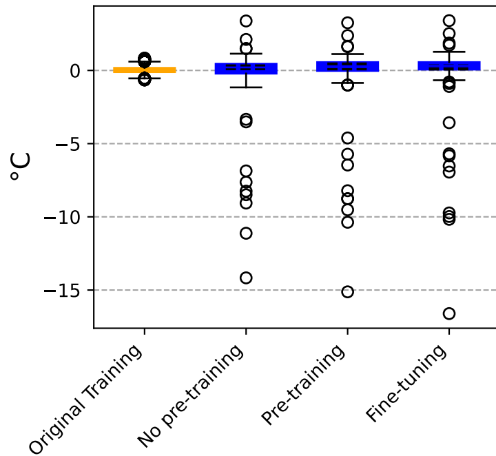
Bias Mean
