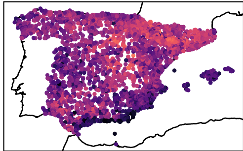
No pre-training
