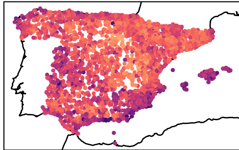
Pre-trained
