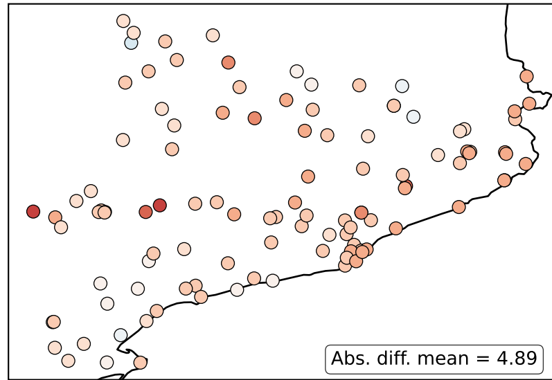
No pre-training
