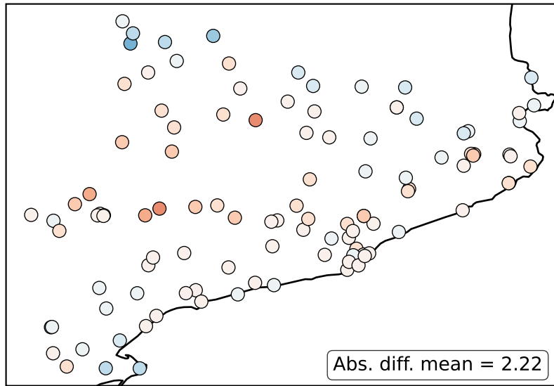
Pre-trained
