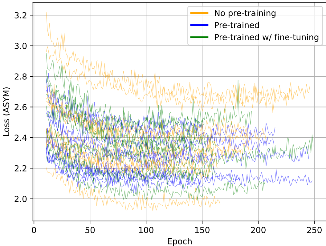
Val - Precipitation
