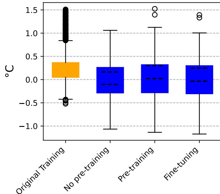
Bias Mean
