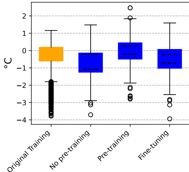
Bias TXx
