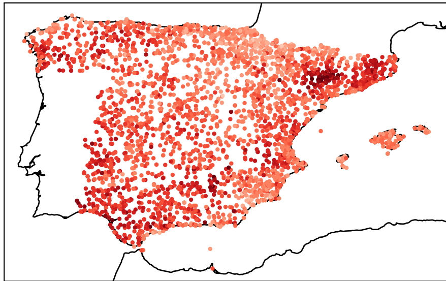
No pre-training
