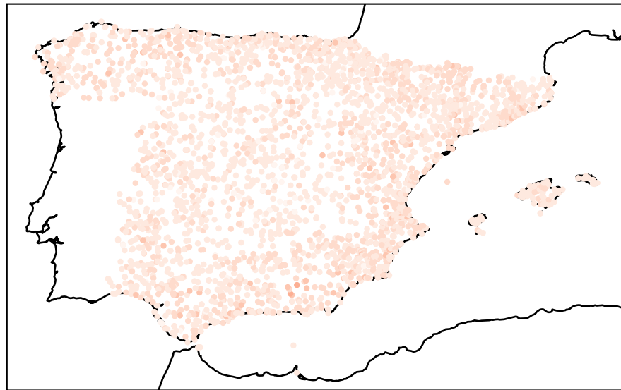
Pre-trained
