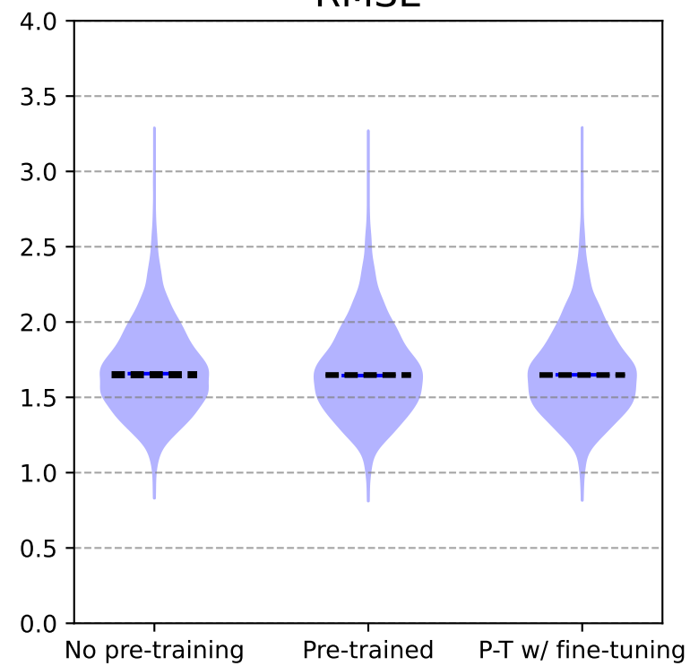
RMSE
