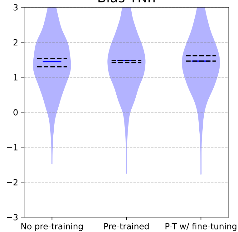
Bias TNn
