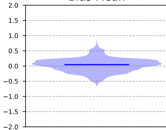
Bias Mean
