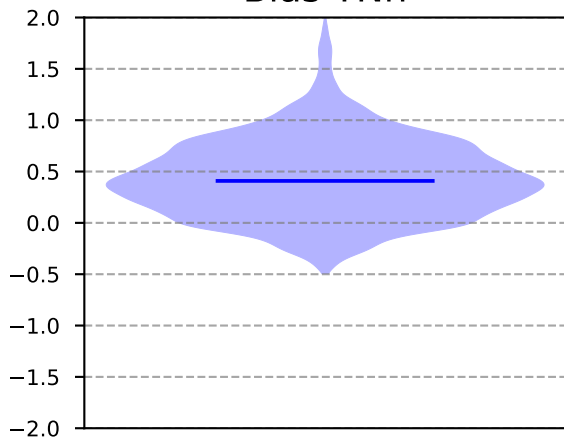
Bias TNn
