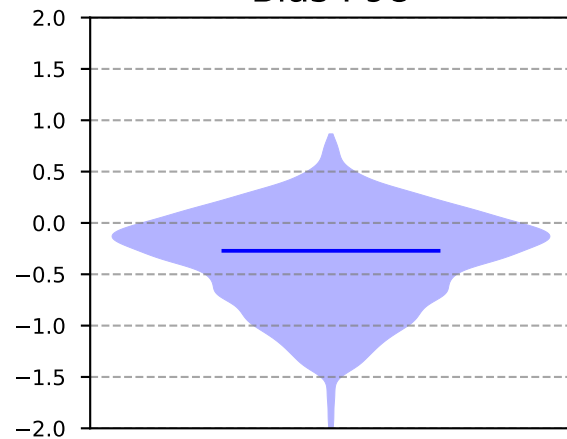
Bias P98
