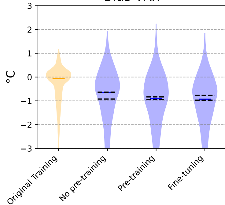
Bias TXx
