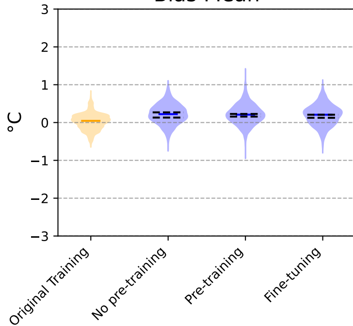
Bias Mean
