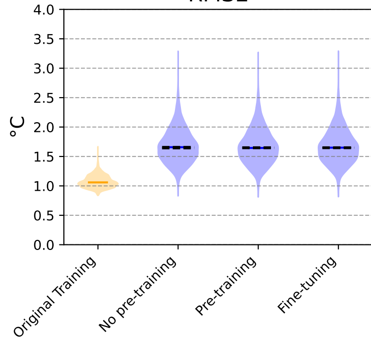
RMSE
