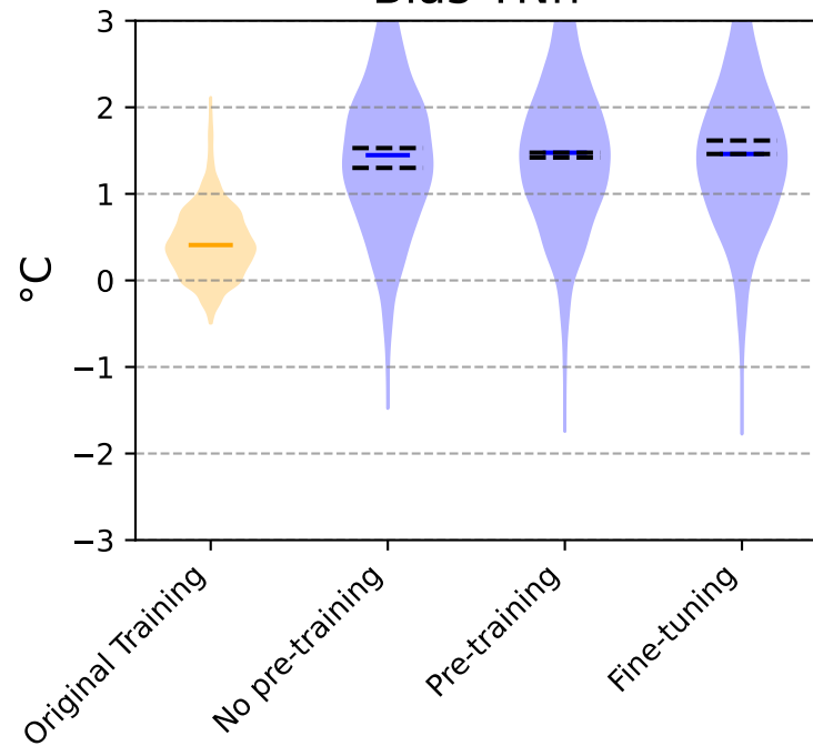
Bias TNn
