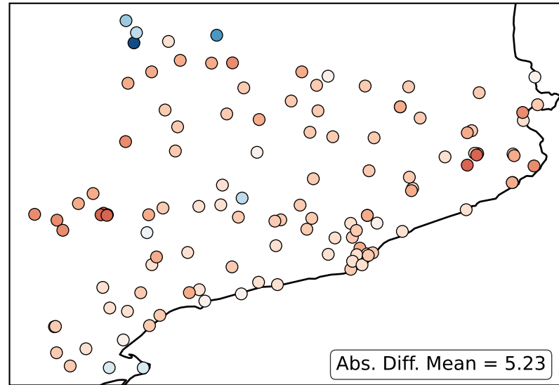
Pre-trained
