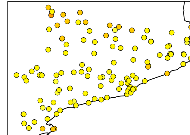
Full fine-tuning
