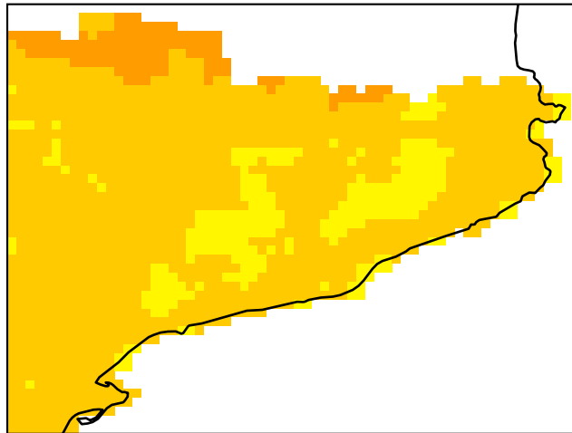
Pre-training
