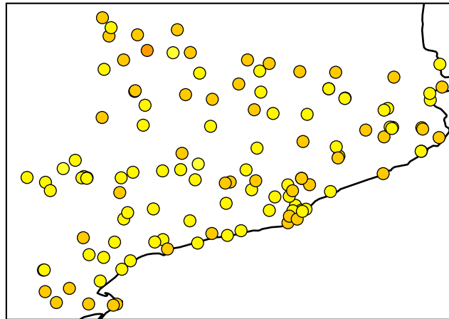
Full-training
