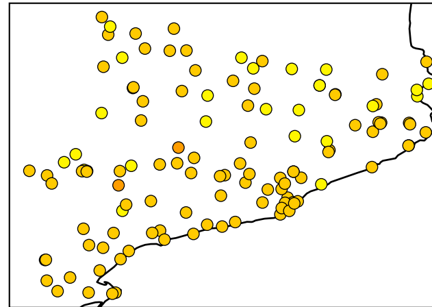
Partial fine-tuning
