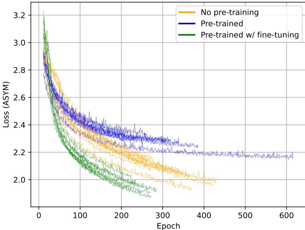
Train - Precipitation
