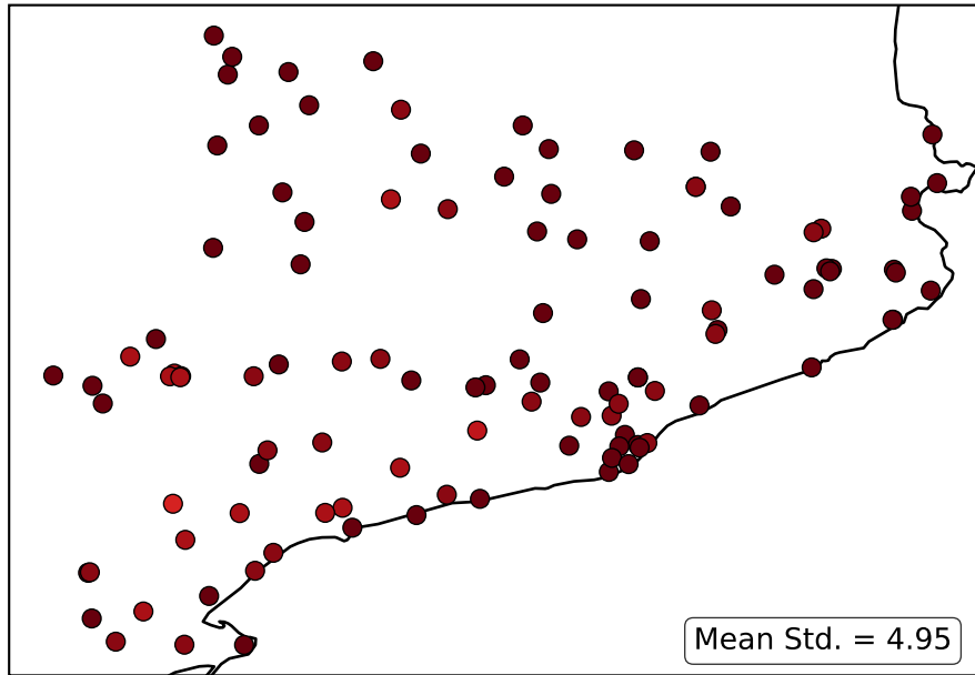
Full-training
