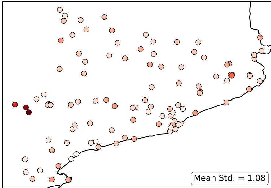
Partial fine-tuning
