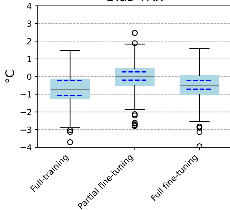
Bias TXx
