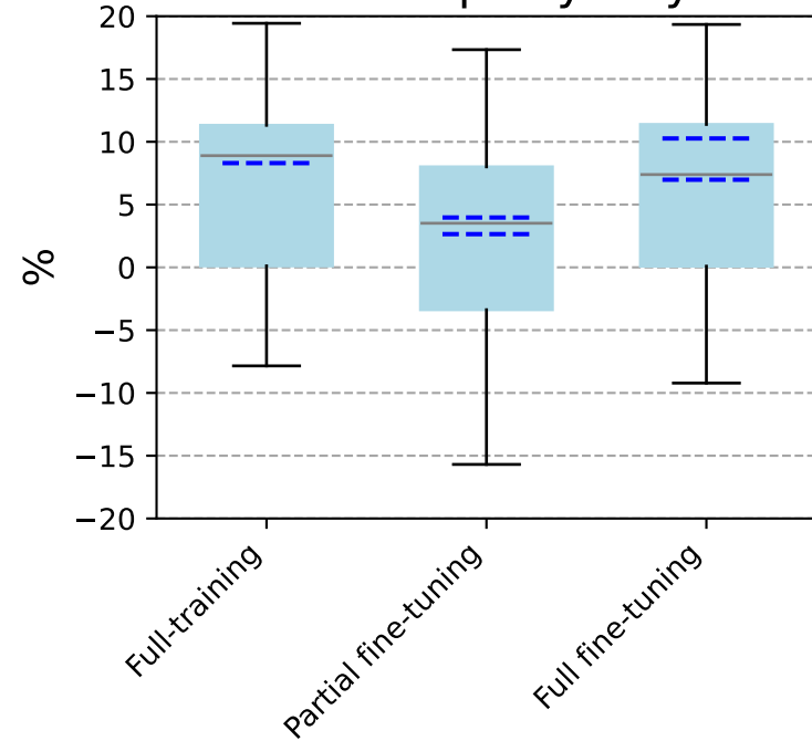
Bias Freq. Dry Days
