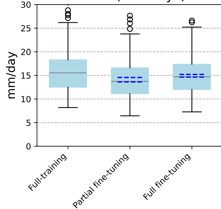
RMSE (wet days)
