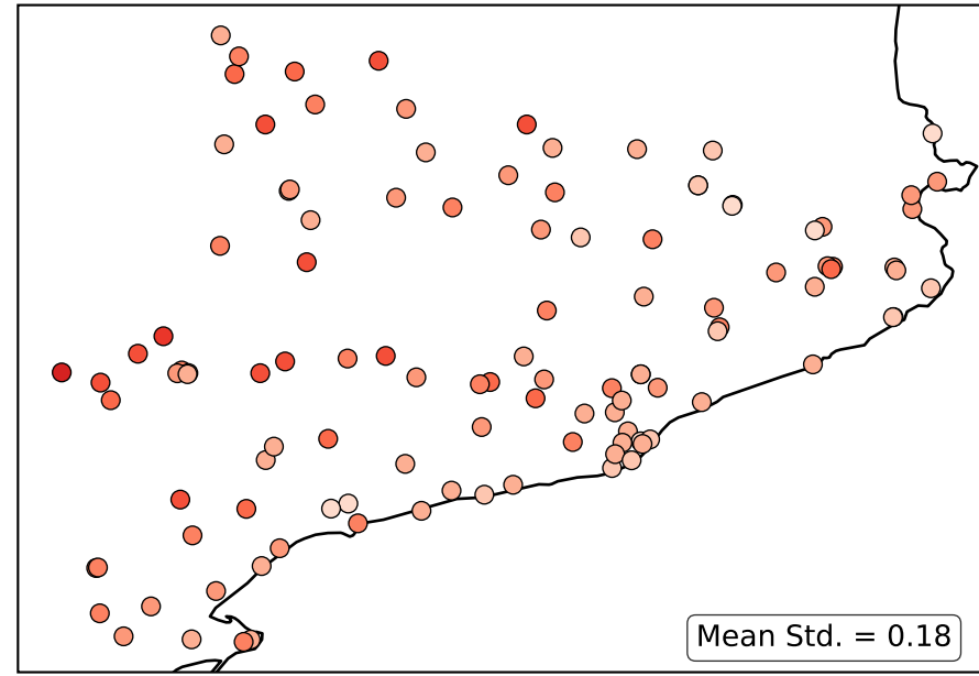
Full fine-tuning
