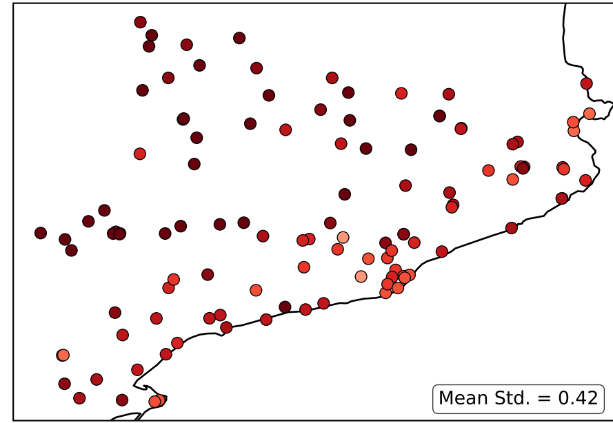
Full-training
