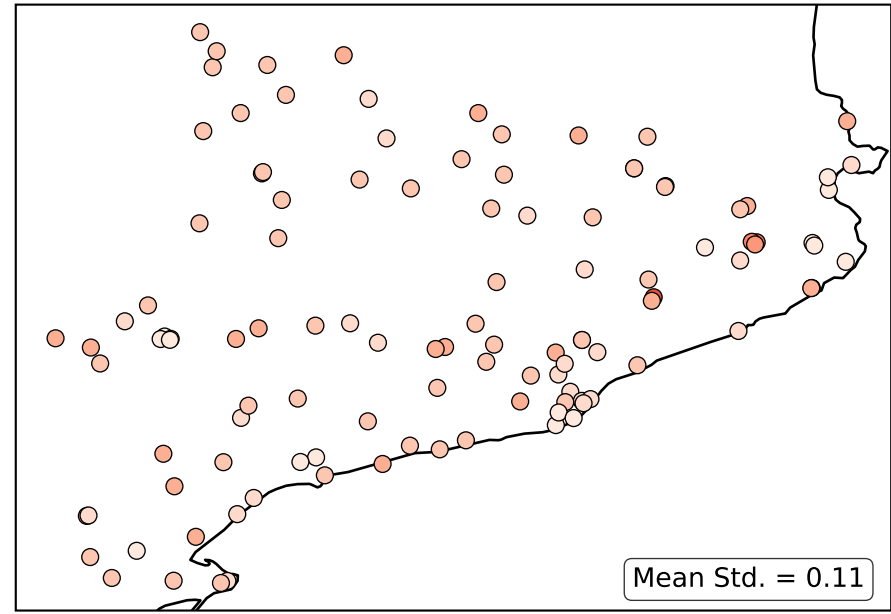
Partial fine-tuning
