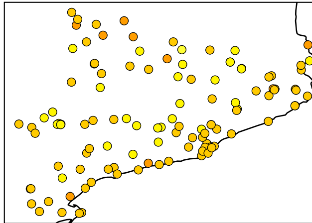
Partial fine-tuning
