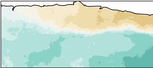
Pre-trained
