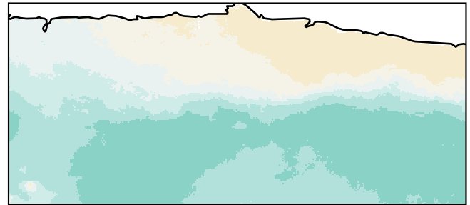
No pre-training
