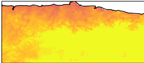
TNn
