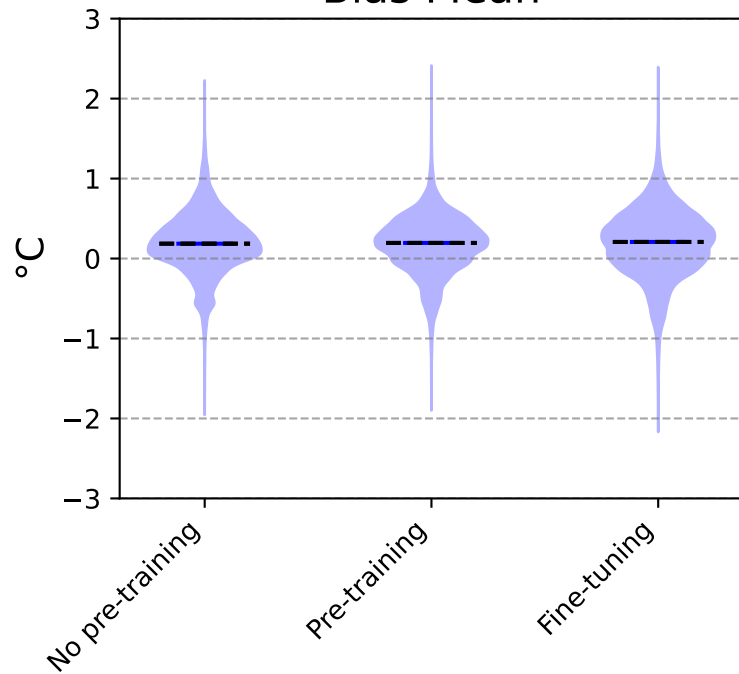
Bias Mean
