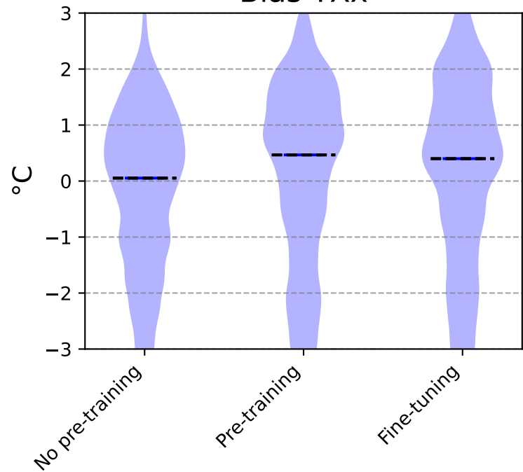
Bias TXx
