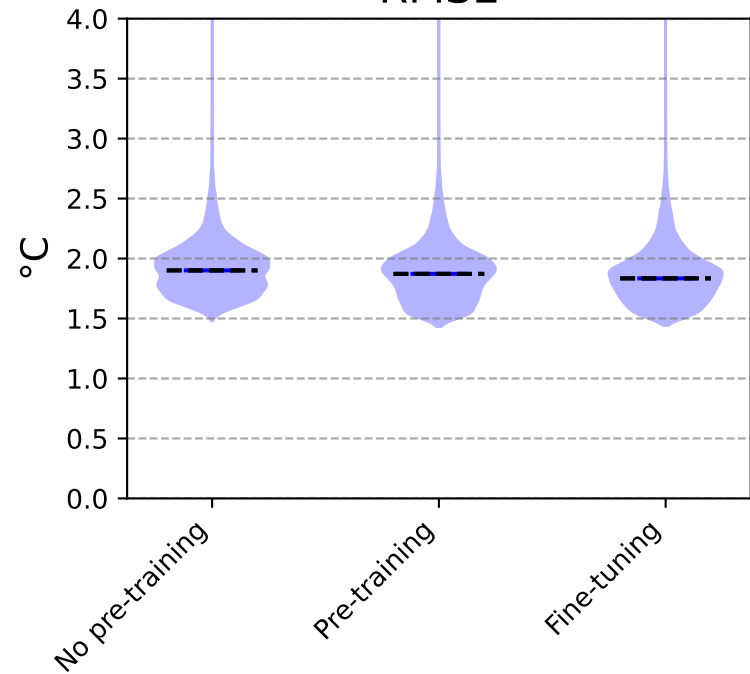
RMSE
