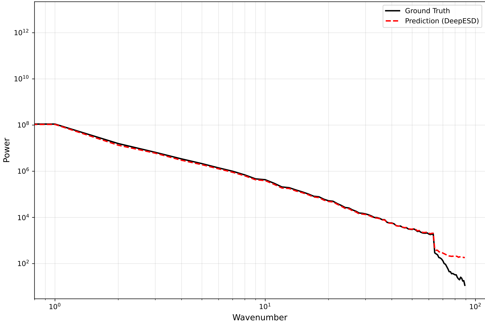
Overall Power Spectral Density | NZ | tasmax
