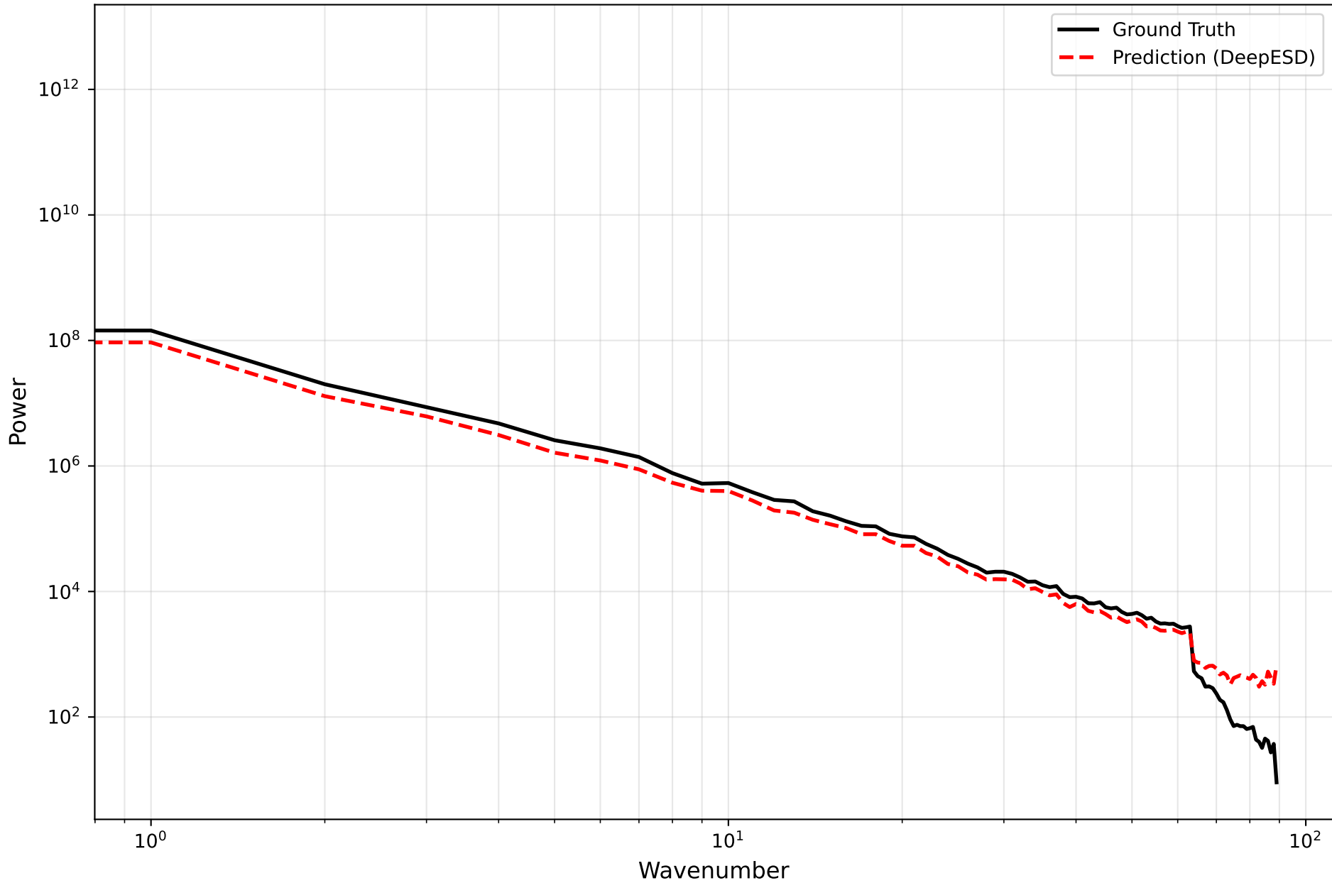
Power Spectral Density | NZ | tasmax | 1980-01-15
