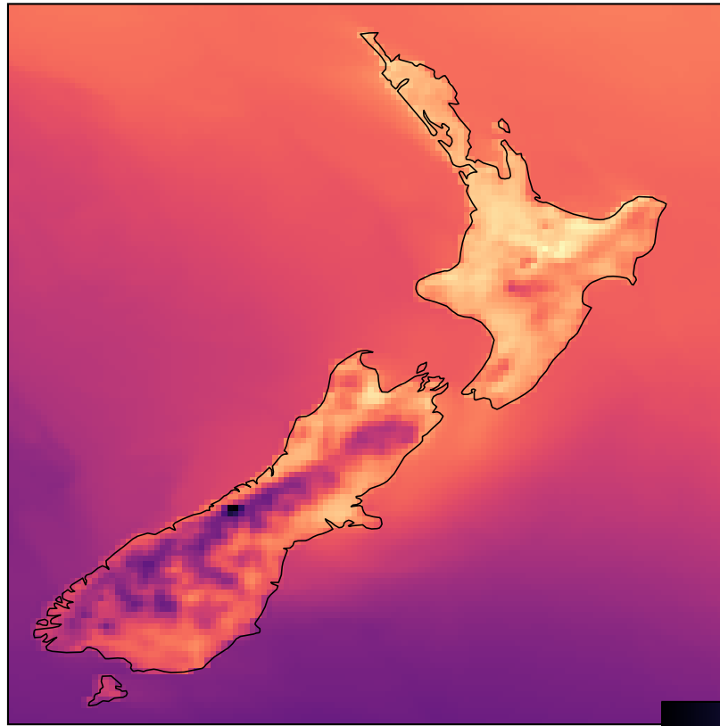
Ground Truth (1980-01-15)
