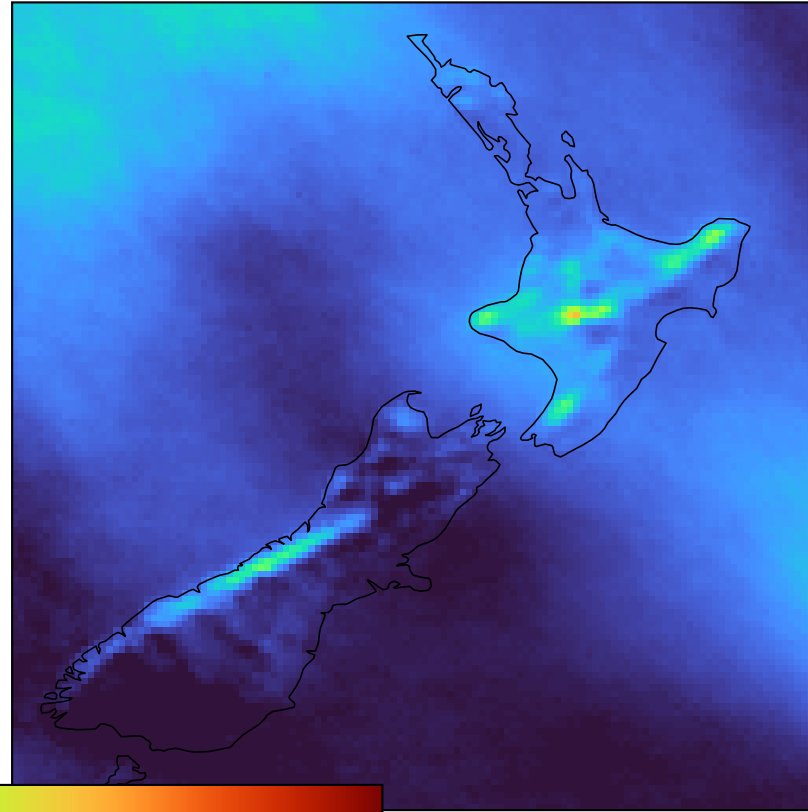
Prediction (DeepESD)
