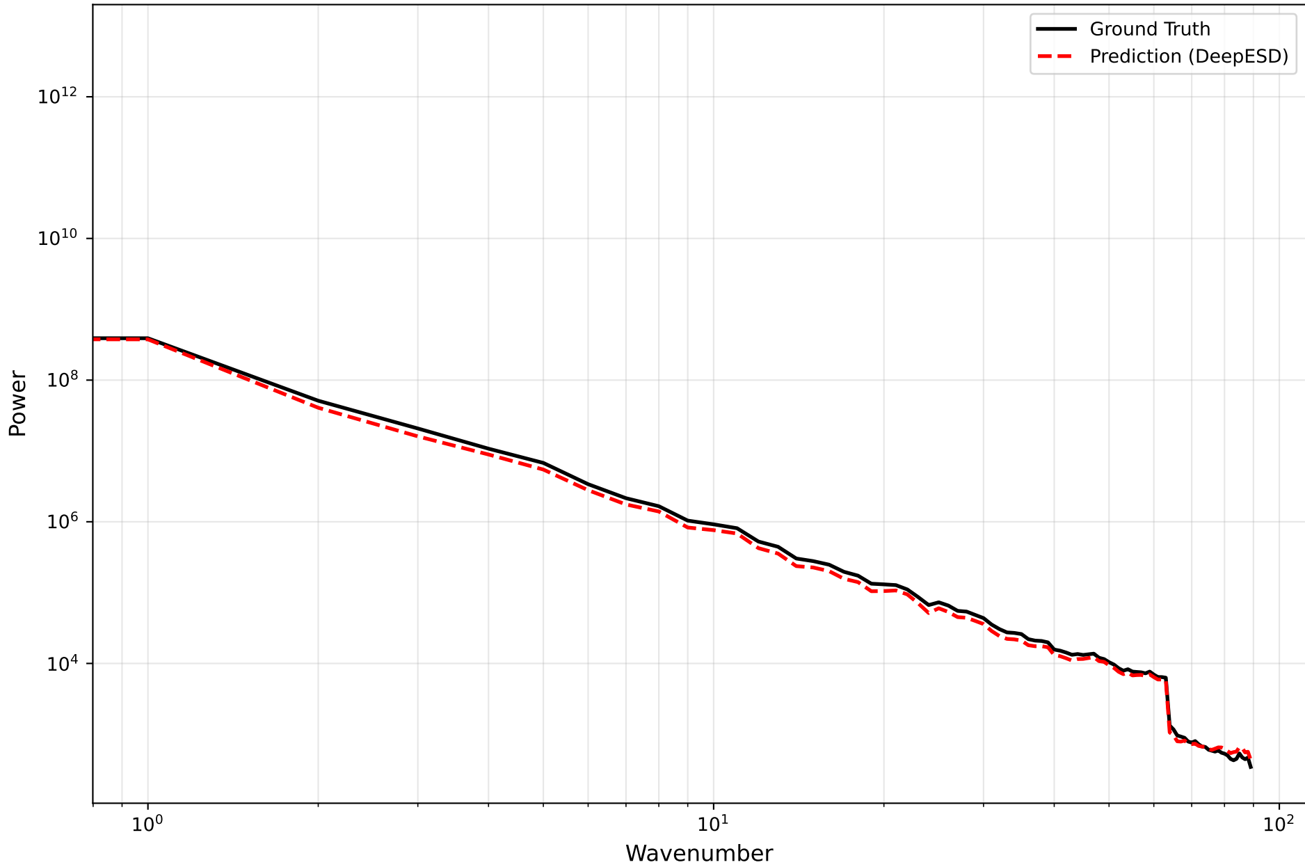
Overall Power Spectral Density | SA | tasmax
