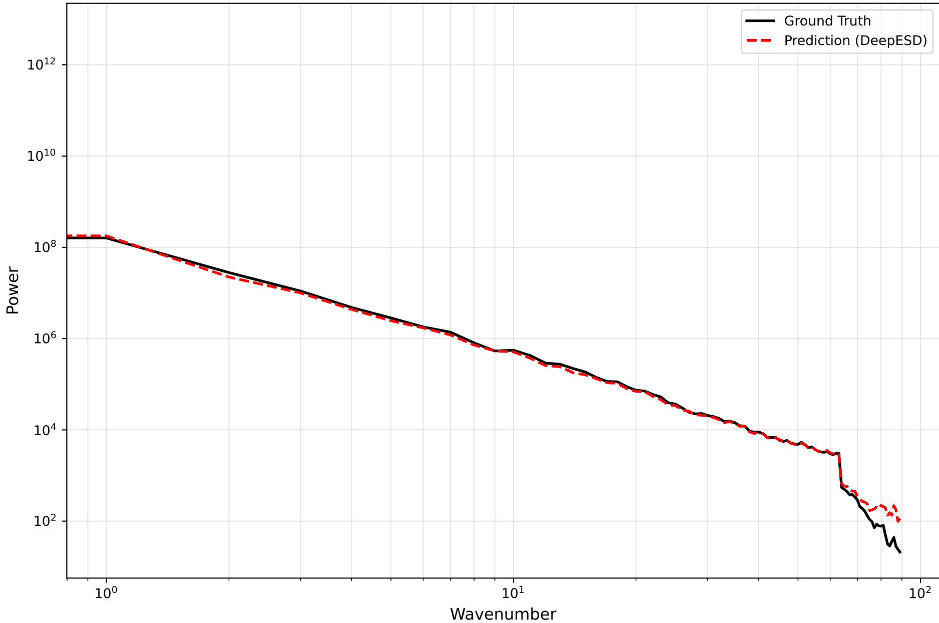
Power Spectral Density | NZ | tasmax | 2098-01-15
