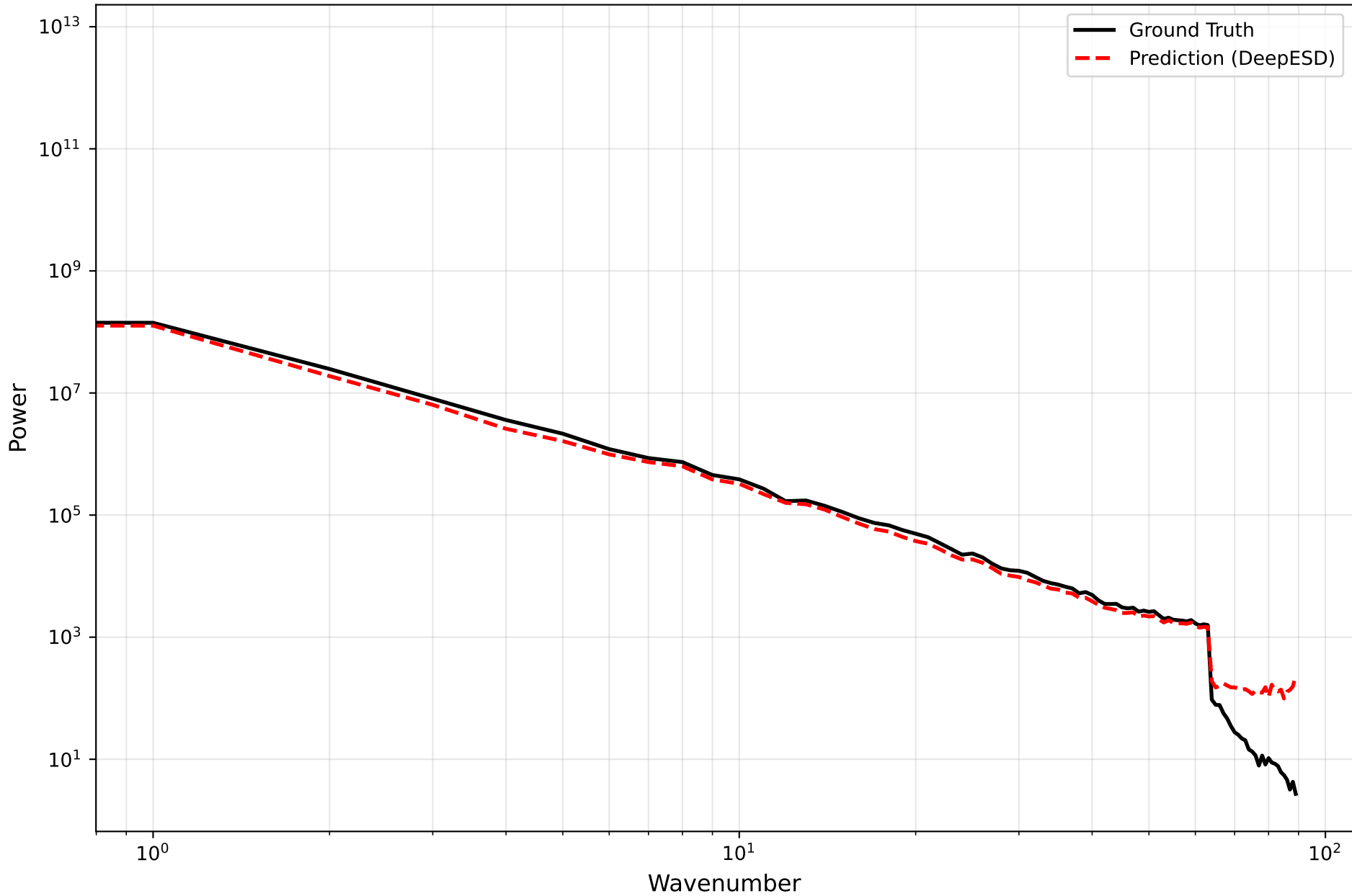
Power Spectral Density | NZ | tasmax | 2098-07-15
