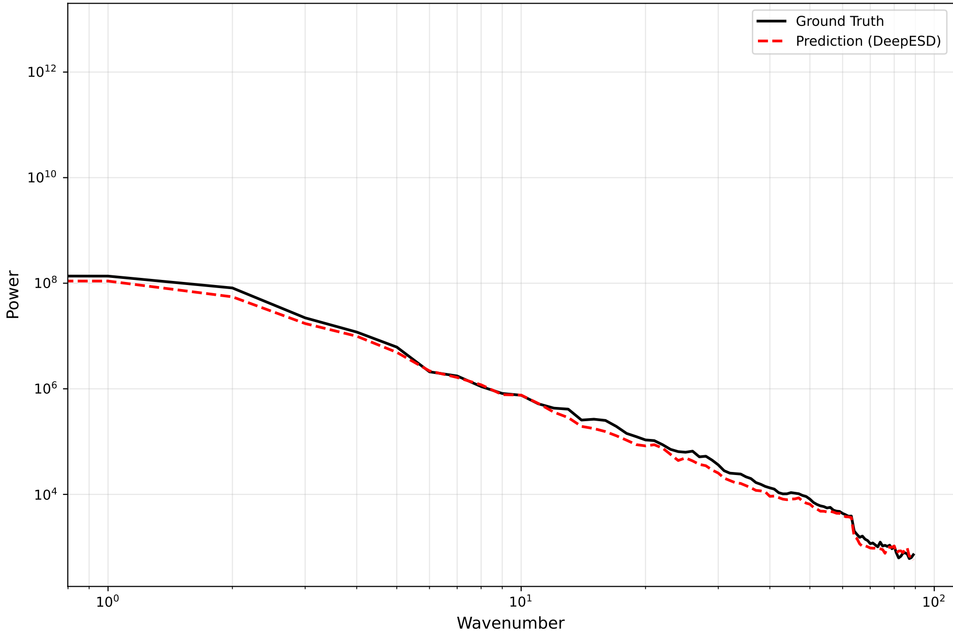
Power Spectral Density | SA | tasmax | 2098-01-15
