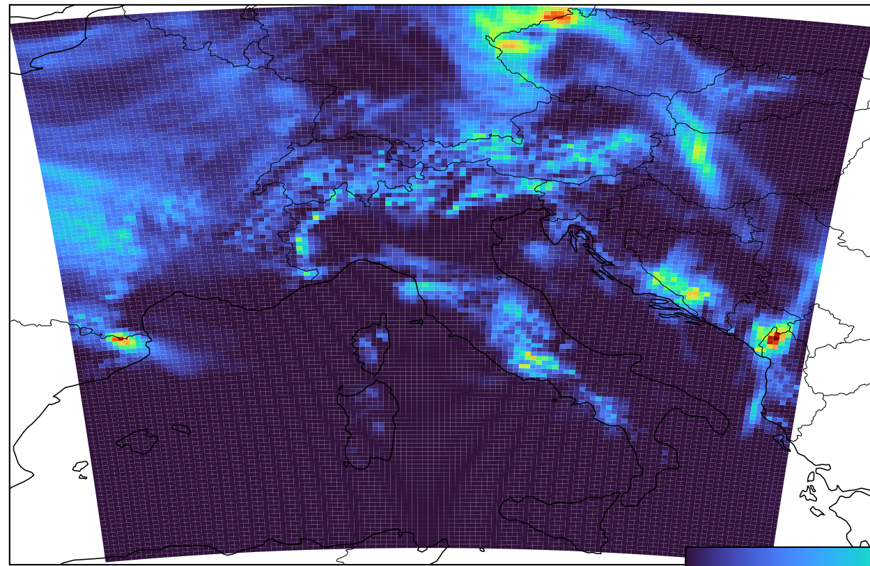
Ground Truth (1980-07-15)
