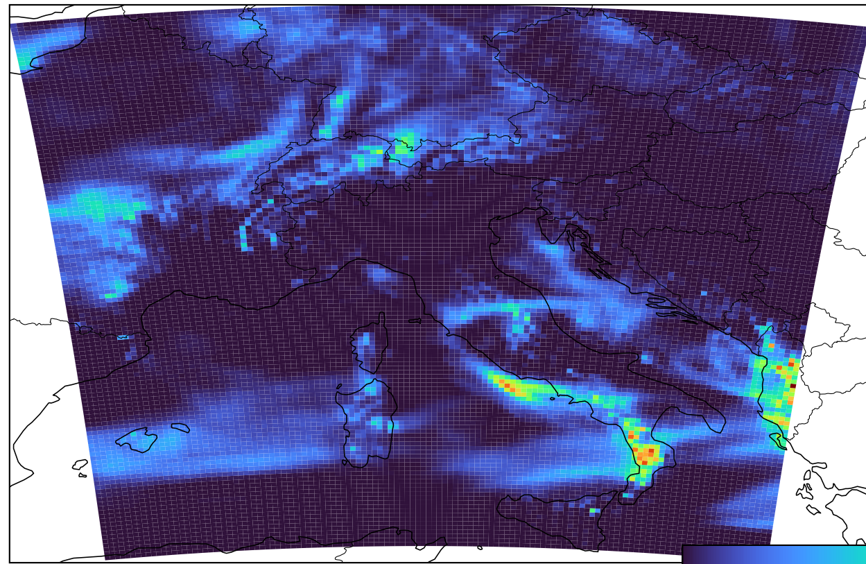
Ground Truth (1980-01-15)
