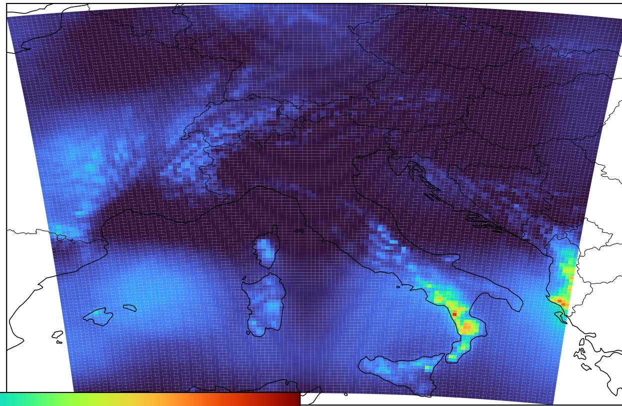
Prediction (DeepESD)
