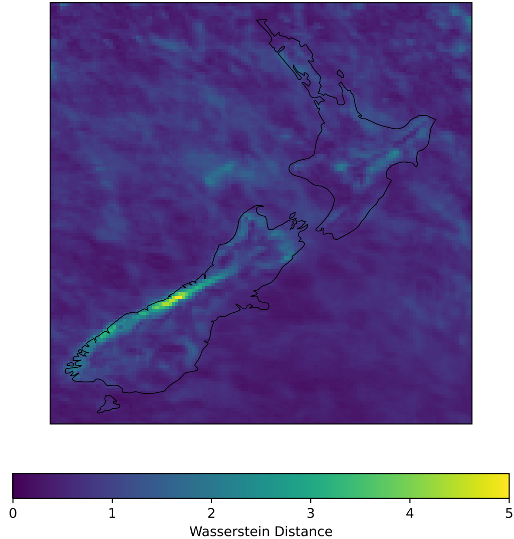
Spatial Map
