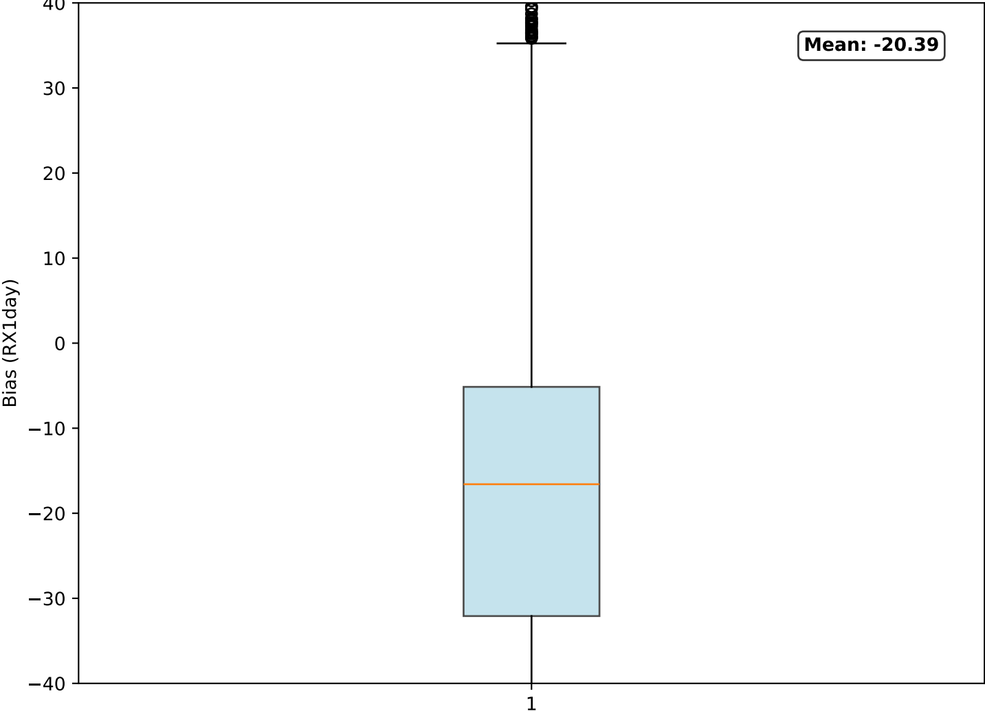
Distribution
