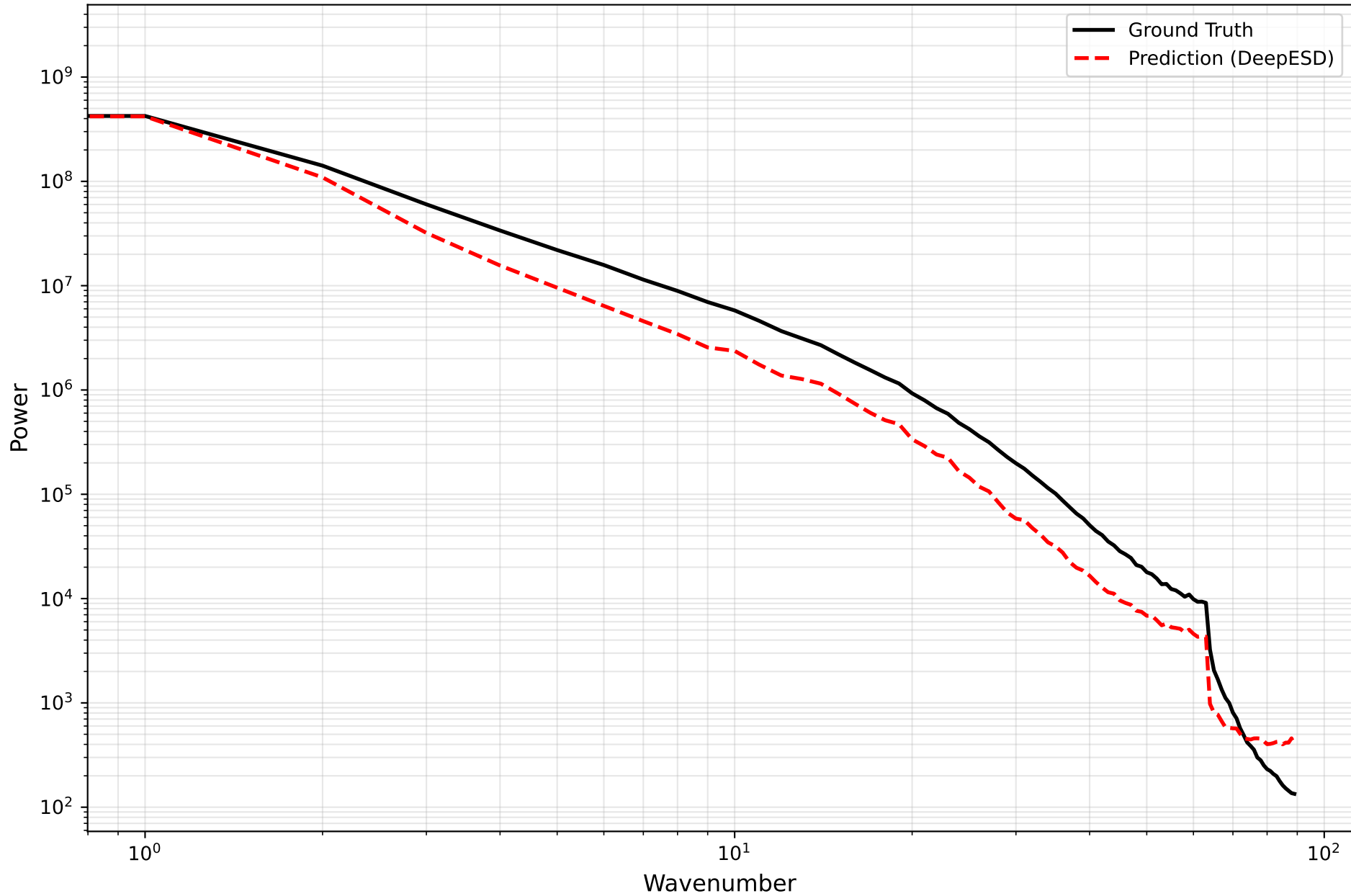
Overall Power Spectral Density | NZ | pr
