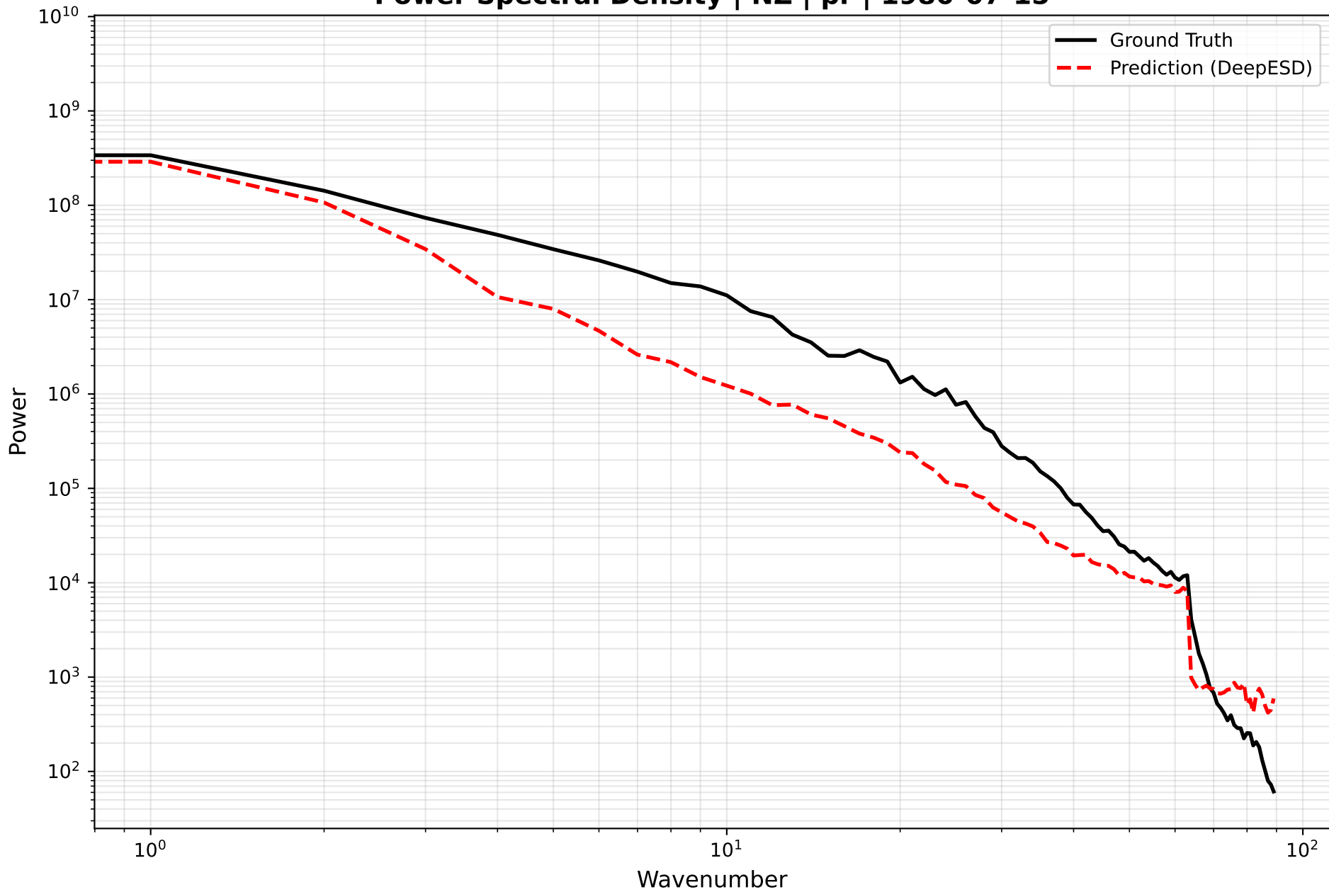
Power Spectral Density | NZ | pr | 1980-07-15
