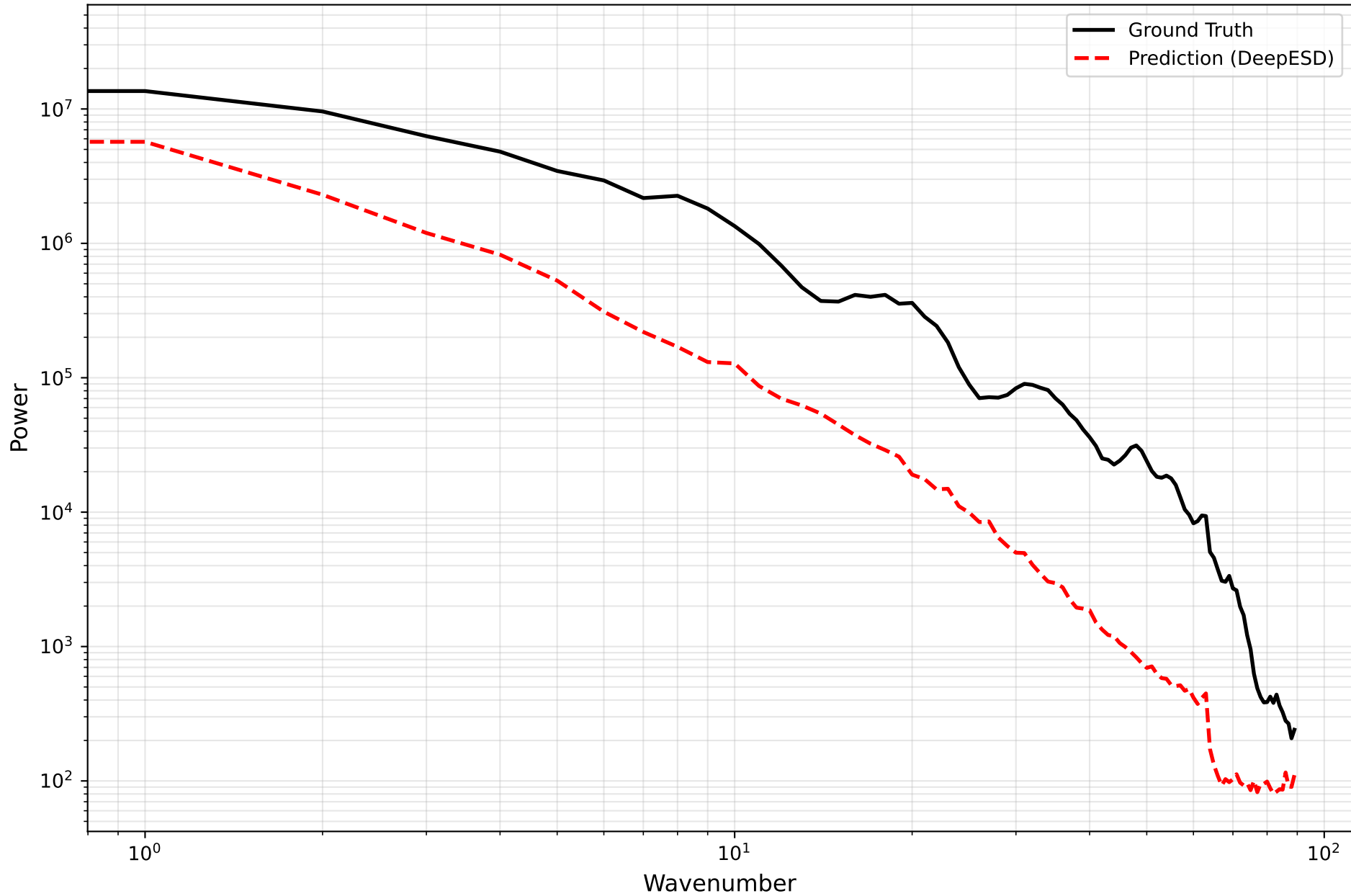
Power Spectral Density | NZ | pr | 1980-01-15
