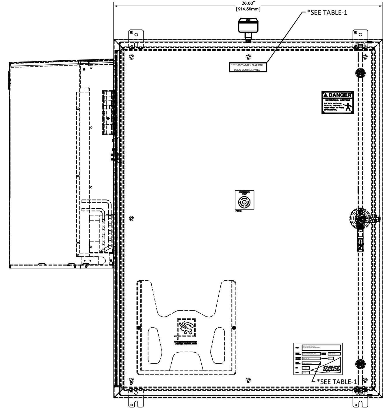
ENCLOSURE LAYOUT NEMA 4X ENCLOSURE TYPICAL OF 2
