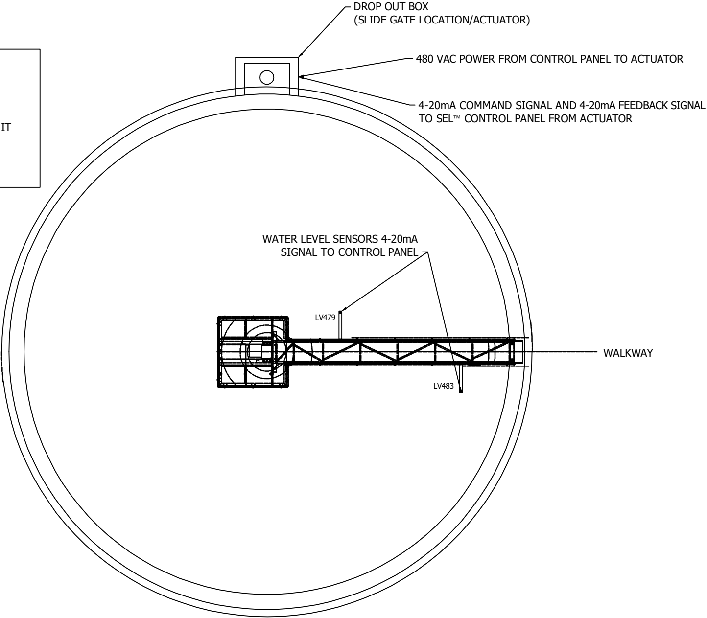
TYPICAL OF SEL™ UNITS
