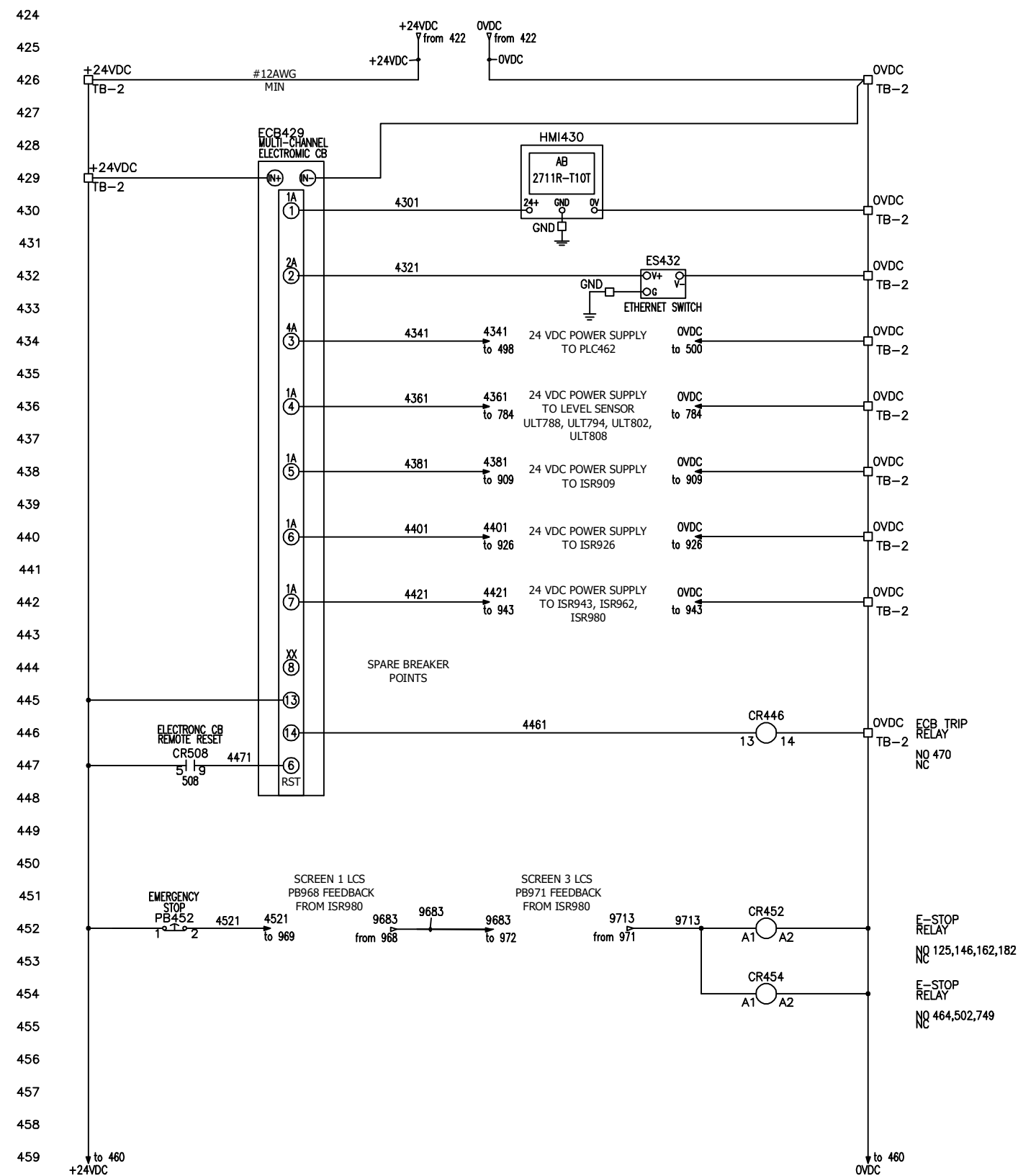
CONTROL POWER SCHEMATIC SHEET 2
