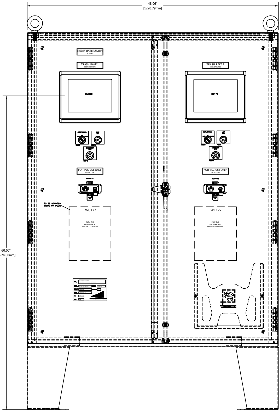
FRONT VIEW
