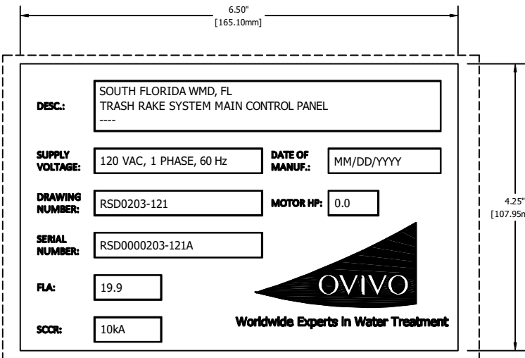
OVIVO NAMEPLATE ENGRAVE AS SHOWN
