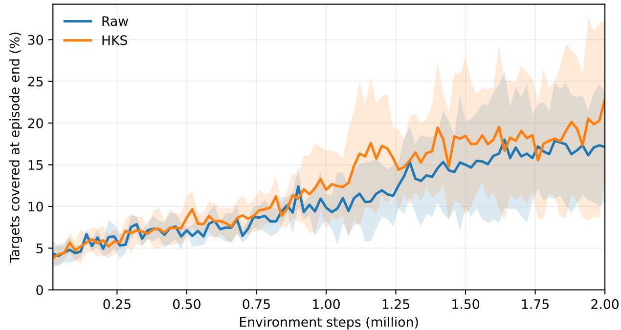
Target coverage during training
