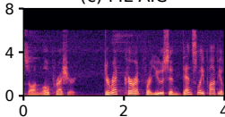
(c) ML-AIC
