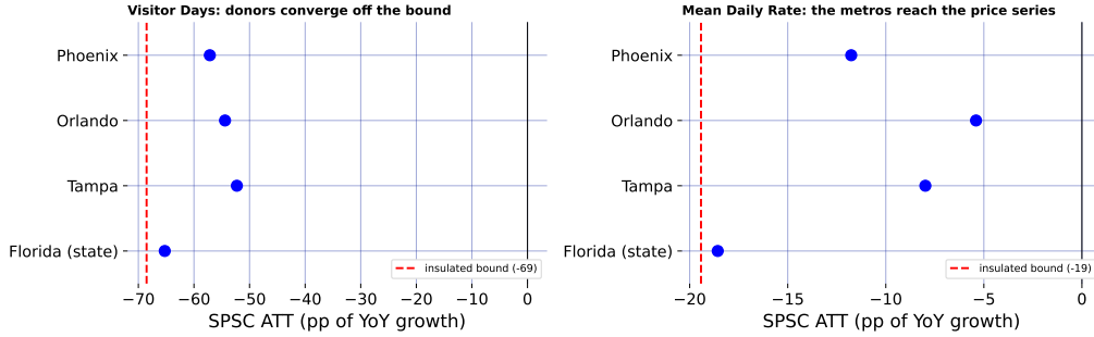
Figure 2: The open-destination ensemble: each donor, fit singly, pulls the estimate off the insulated-only bound.
