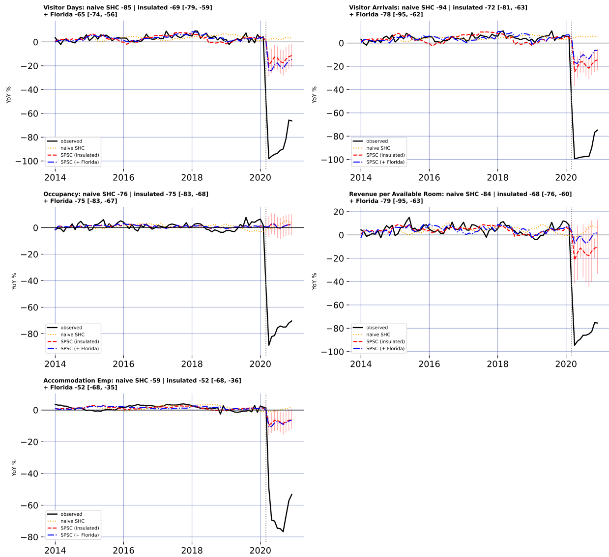
Figure 1.5: Observed, naive SHC, and both proximal SPSC counterfactuals for five headline outcomes.
