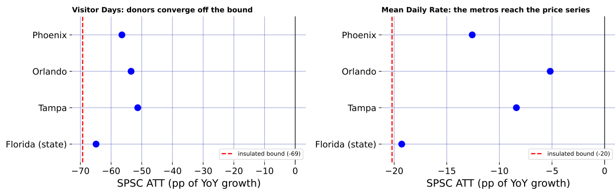
Figure 1.4: The open-destination ensemble: each donor, fit singly, pulls the estimate off the insulated-only bound.
