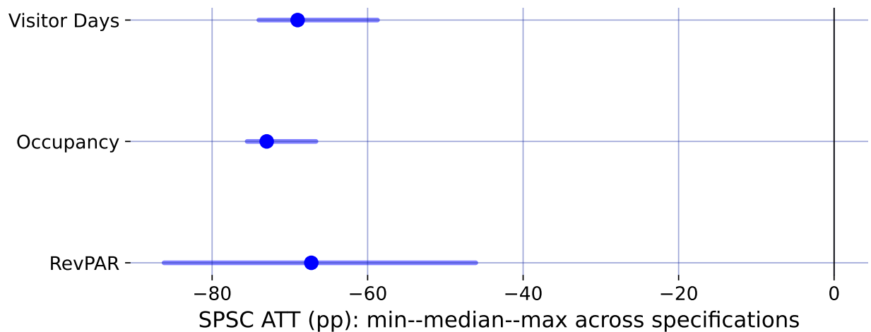
Figure 1.3: Specification robustness band: median SPSC ATT (point) and min-max range across seven specifications.
