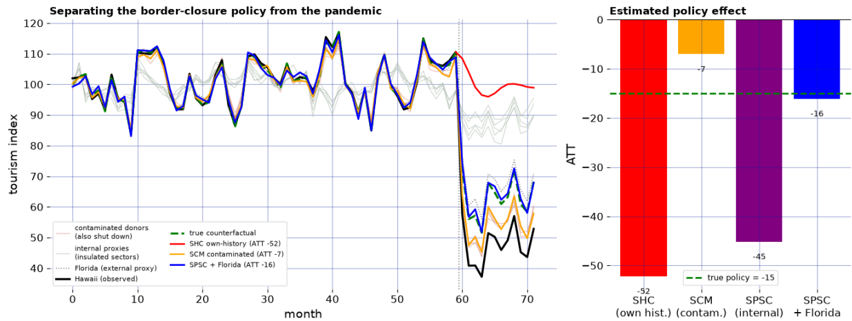
Figure 1.1: The fan experiment with a known answer. A synthetic Hawaii-like economy is stirred by an ordinary business cycle (the house thermostat) and, after month 60, a sharp pandemic-style collapse (the breeze); a border-closure policy (the fan) with a true effect of -15 points is layered on. Left: the observed treated series (black) falls below its true no-policy counterfactual (green dashed) by the policy effect; the own-history reconstruction (red) is blind to the breeze, the contaminated-donor comparison (orange) tracks rooms that also ran fans, and Single Proxy Synthetic Control with the external Florida window (blue) hugs the truth. Right: each method's estimated policy effect against the true -15 (green dashed). The two naive methods miss in opposite directions; the proximal estimate, built on a valid external negative control, recovers the answer. The panel shows the single draw quoted in the text; averaged over repeated draws the estimates are close and the ordering is unchanged.
