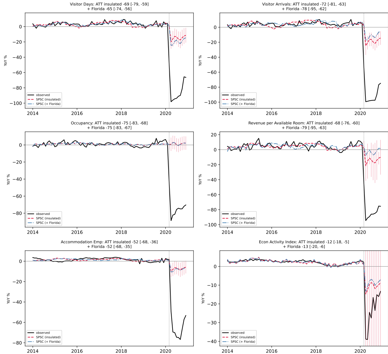
Figure 1.6: SPSC counterfactuals for the six headline outcomes: observed (black), the insulated-donor counterfactual (dashed), and the counterfactual after adding the Florida travel-demand donor (dash-dot). Red spikes are the per-period conformal prediction interval around the insulated counterfactual (clipped to each panel; wide/degenerate for the near-interpolating series, where the ATT interval is the informative uncertainty). Each panel title gives the ATT with its 95% GMM confidence interval for both donor sets.
