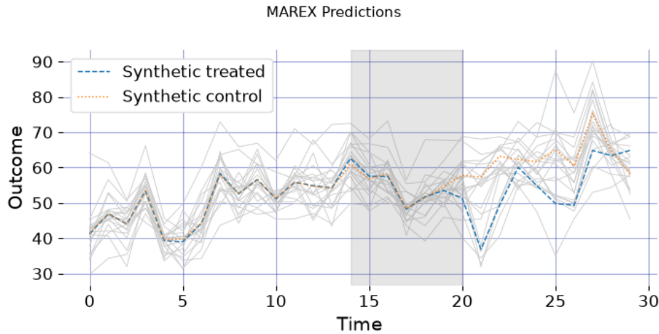
Figure 5: MAREX’s own design diagnostic, drawn by the library, for Apple’s go-dark test – a reproduction of Abadie and Zhao’s Figure 4. The faint lines are the individual DMAs; the dashed and dotted series are the synthetic treated and synthetic control the design built from pre-launch sales alone. They track through the fitting window and the shaded blank weeks, then separate once paid media goes dark at week 20 – the gap is the sales the dark markets forgo, which is what the advertising had been generating.
