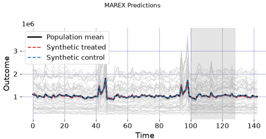
Figure 7: MAREX’s own design diagnostic, drawn by the library, for the Walmart placebo experiment, reproducing Abadie and Zhao’s Figure 2. The red and blue dashed lines are the synthetic treated and synthetic control units the design built from the pre-experimental window; the faint lines are the individual stores. The two synthetics track each other through the fitting and blank weeks and stay close after the fictitious intervention at week 129: the design produces no spurious effect.
