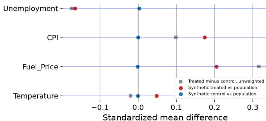
Figure 6: Covariate balance for the chosen design (a love plot), one row per store-level covariate. Grey squares are the raw standardized difference between the two treated stores and the controls before weighting; the red and blue dots are the synthetic treated and synthetic control, each against the population. The synthetic control (blue), free to draw on all forty-three remaining stores, sits on the population; the synthetic treated (red), restricted to two stores by the cardinality constraint, is pulled most of the way from the raw split toward balance.
