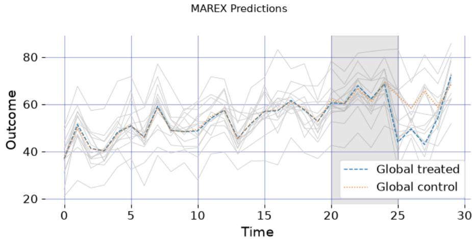
Figure 5: MAREX’s own design diagnostic, drawn by the library, with the donor cloud overlaid – a reproduction of Abadie and Zhao’s Figure 4. The faint lines are the individual simulated markets; the bold dashed and dotted series are the synthetic treated and synthetic control the design built from pre-experiment data alone. They track through the fitting window and the shaded blank periods, then separate after the experiment begins at week 25 as the treated markets realize their treated outcomes – the gap being the estimated effect.
