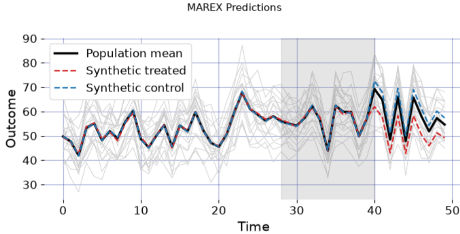
Figure 5: MAREX’s own design diagnostic, drawn by the library, for Apple’s go-dark test, a reproduction of Abadie and Zhao’s Figure 4. The thick solid line is the population mean; the red and blue dashed lines are the synthetic treated and synthetic control markets (the dark and the lit DMAs) the design built from pre-launch sales alone; the faint lines are the individual DMAs. The synthetics track the population through the fitting window and the shaded blank weeks, then the treated series separates once paid media goes dark at week 40. That gap is the sales the dark markets forgo, which is what the advertising had been generating.
