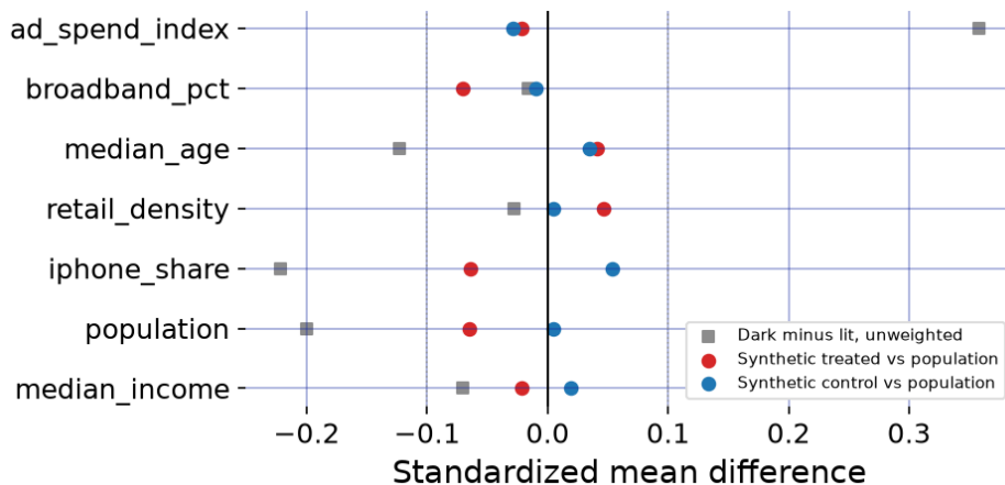
Figure 4: Covariate balance for the chosen design (a love plot), one row per market trait. Grey squares are the raw standardized difference between the darkened and lit markets before weighting; the red and blue dots are the synthetic treated and synthetic control, each against the population. The raw split is off by up to a third of a standard deviation, but MAREX pulls both synthetics onto the population, well inside the dotted 0.1 guides: the design is balanced before the test begins.
