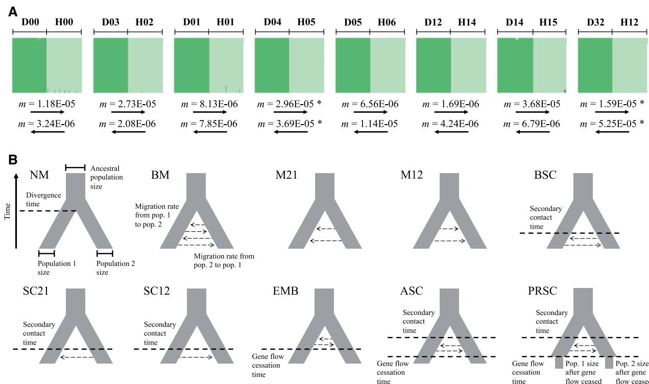
FIG. 4. Patterns of gene flow and admixture between parapatric Dune–Headland populations. (A) Bayesian assignment of individuals to genetic clusters within STRUCTURE for K = 2 for the Dune (dark green) and Headland (light green) ecotypes at each locality. Each individual is depicted as a bar, with colors representing ancestry proportions to each cluster. Below are the migration rates ( m , backward in time) for the most likely divergence model for Dune to Headland, and Headland to Dune within each locality estimated within fastsimcoal2 . Asterisks denote pairs with 2Nm > 1 . (B) Schematic diagram representing the ten demographic models run in fastsimcoal2 and their estimated parameters: no migration (NM), bidirectional migration (BM), population 2 to population 1 migration (M21), population 1 to population 2 migration (M12), bidirectional migration after secondary contact (BSC), population 2 to population 1 migration after secondary contact (SC21), population 1 to population 2 migration after secondary contact (SC12), bidirectional migration after population splitting with cessation of gene flow (EMB), ancient bidirectional secondary contact (ASC), population size reduction after bidirectional secondary contact (PRSC).
