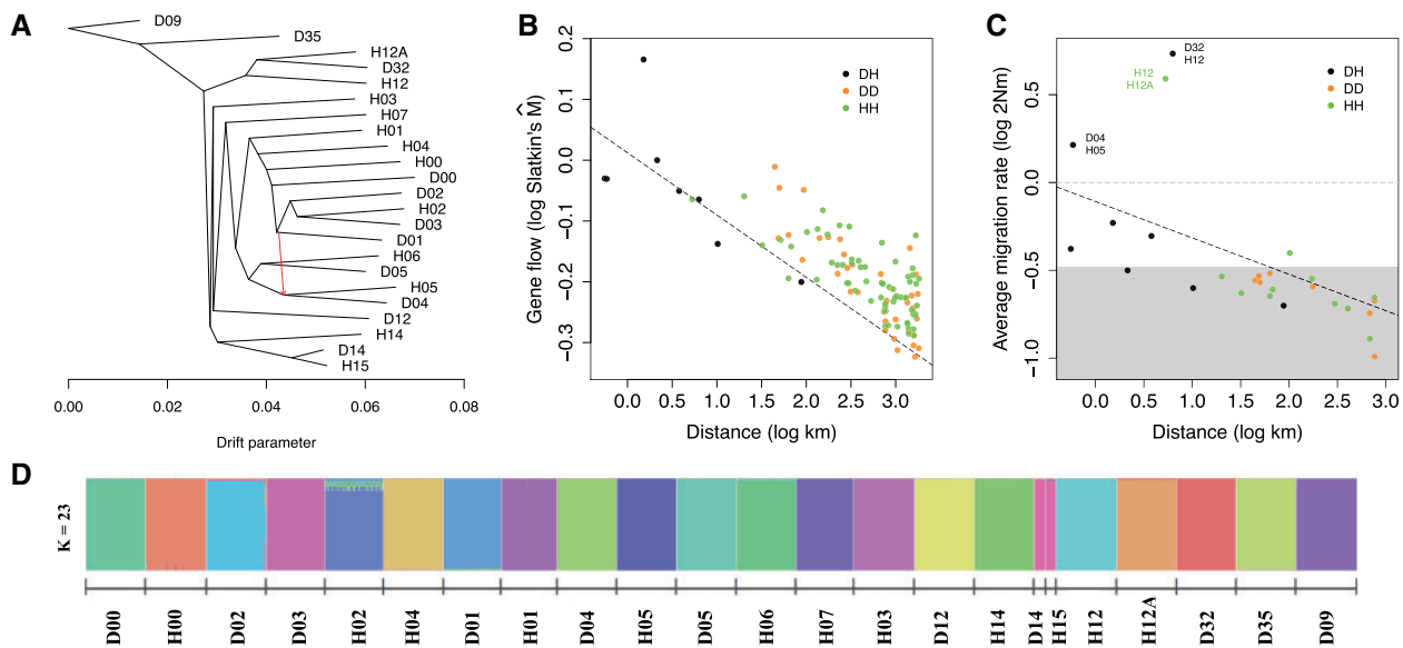
FIG. 3. Patterns of long-distance gene flow, isolation by distance, and genetic clustering. (A) Maximum likelihood tree with one migration event inferred in TreeMix , the x -axis representing genetic drift. The red arrow represents the migration event ( w = 0.40 ). (B) Patterns of IBD using Slatkin's \hat{M} for parapatric Dune–Headland (black), Dune–Dune (orange), and Headland–Headland (green) pairs. Black dashed line represents the linear model for the DH comparisons. (C) Patterns of IBD across Dune and Headland populations for Dune–Headland (DH, black), Dune–Dune (DD, orange), and Headland–Headland (HH, green) pairs. Average migration rate is the mean bidirectional migration for each pair estimated in fastsimcoal2 . Gray shading represents the null expectation for migration rates, inferred from the maximum migration value from three allopatric comparisons ( 2Nm = 0.33 ). Gray horizontal dashed line represents one migrant per generation ( 2Nm = 1 ). Pairs falling above this line are labelled. Black dashed line represents the linear model for the DH comparisons. (D) Bayesian assignment of individuals to genetic clusters within fastSTRUCTURE for K = 23 . Each of the 1,319 individuals is depicted as a bar, with colors representing ancestry proportions to each cluster. Populations are ordered according to their geographic distribution along the coast.
