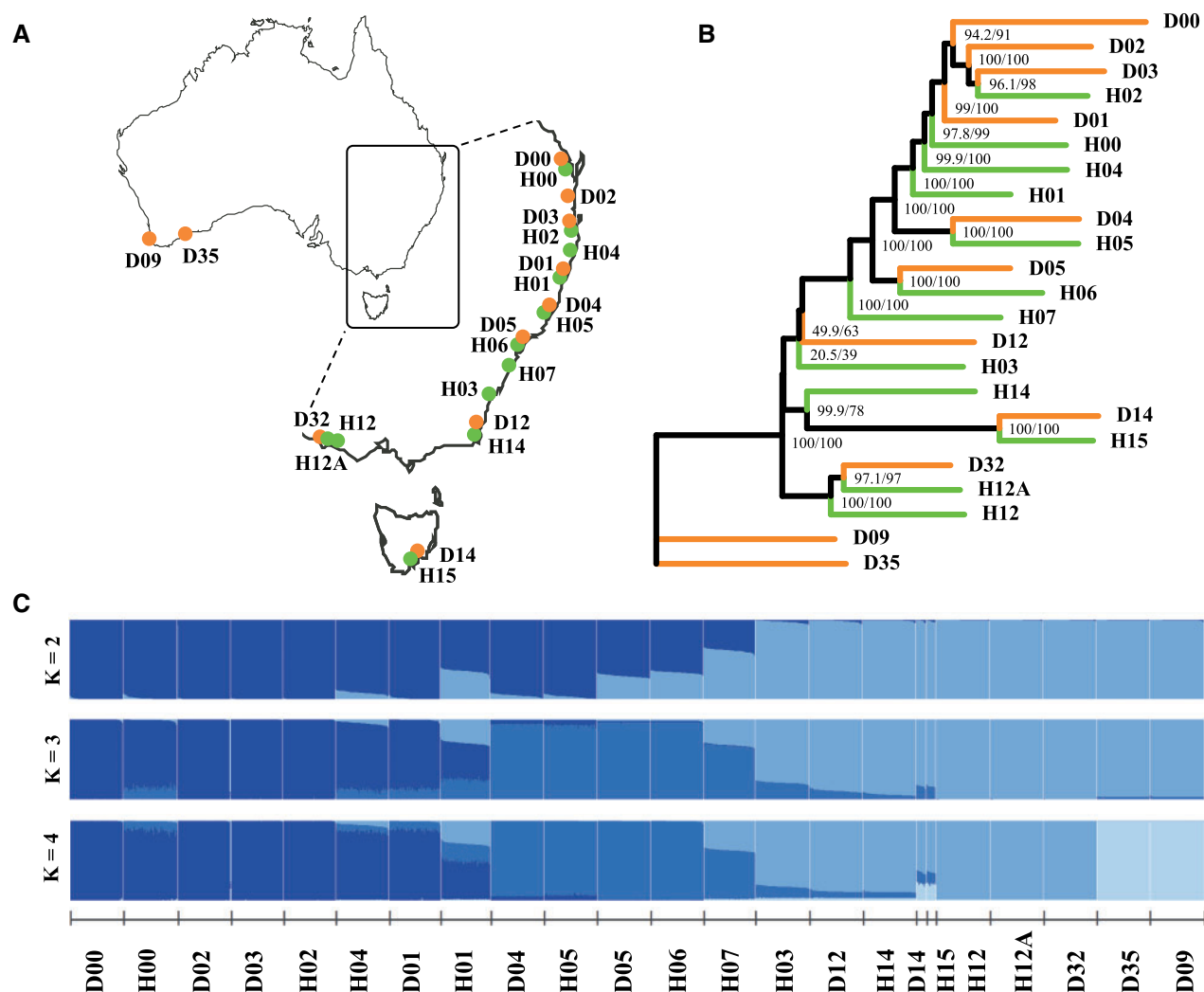
Fig. 2. Sampling locations and genetic clustering of Senecio laetus populations. (A) Sampling locations of the 23 Dune (orange) and Headland (green) S. laetus populations along the coast of Australia. (B) Maximum likelihood phylogeny of Dune and Headland populations implemented in IQ-TREE . Numbers on each node represent the SH-aLRT support (%), followed by the ultrafast bootstrap support (%). (C) Bayesian assignment of individuals to genetic clusters within fastSTRUCTURE for K = 2-4 . Each of the 1,319 individuals is depicted as a bar, with colors representing ancestry proportions to each cluster. Populations are ordered according to their geographic distribution along the coast.
