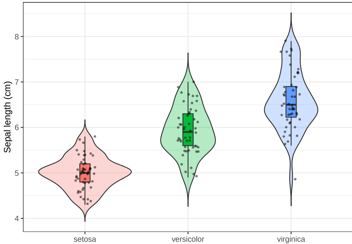
Sepal Length by Species
